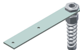
straight mounting bracket for spiral cable, 160x25mm incl. spiral cable gland M16 (roller shutters)
